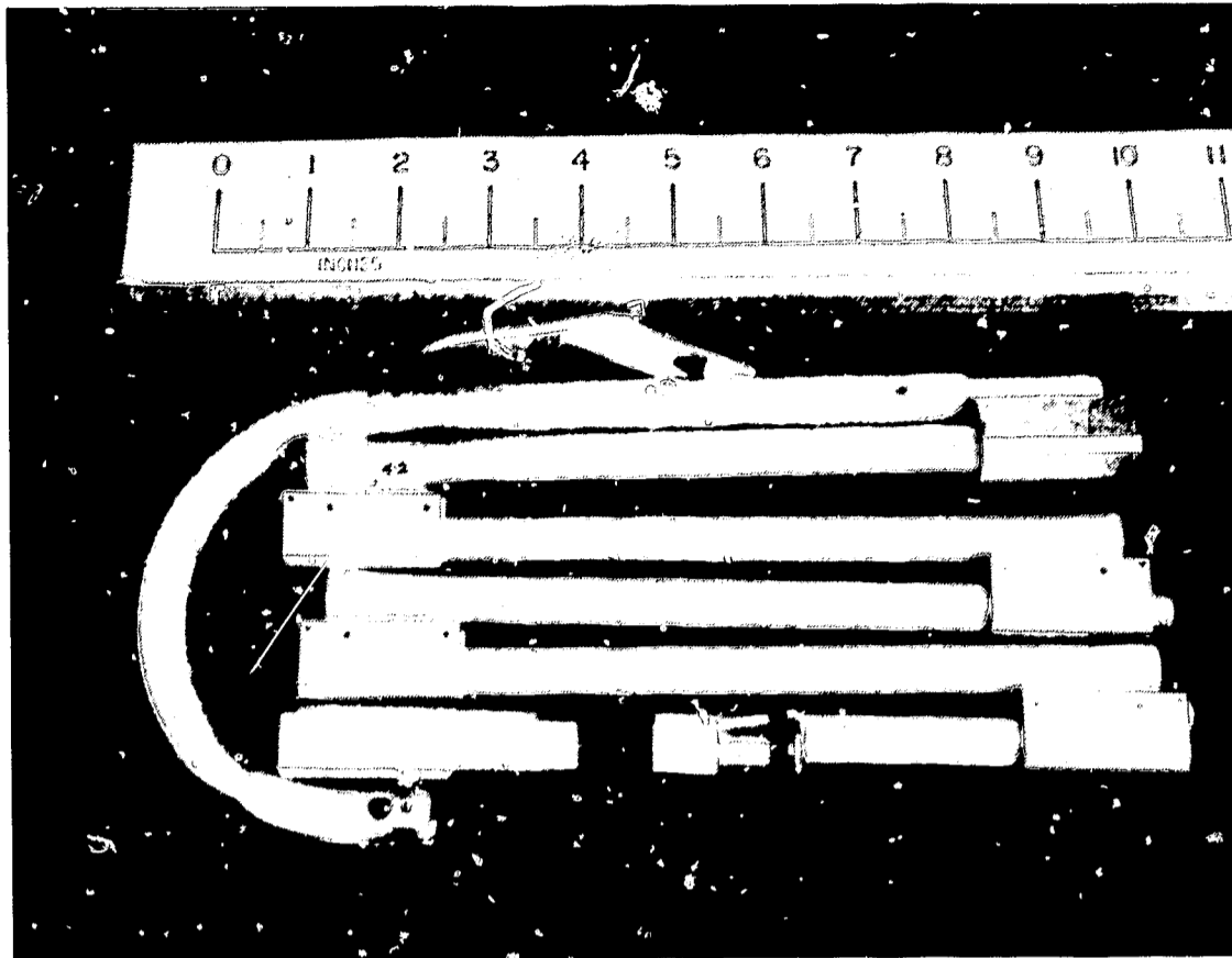
FIG. 3. Center's 55" long swaged tube, central steel cable, collapsible cane with hinges shown folded for storage.
